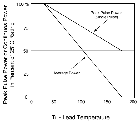
Fig. 4 - Derating Curve
